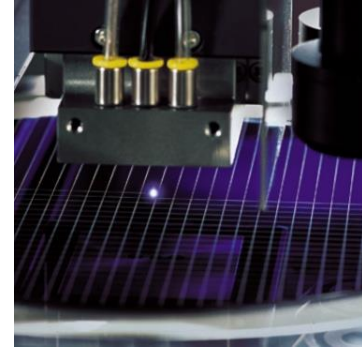
WAFER SINGULATION
