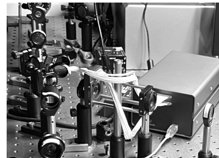
Self-built microscopes
