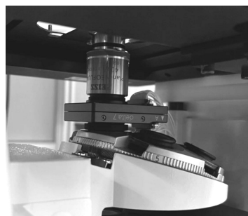
Turret mount
