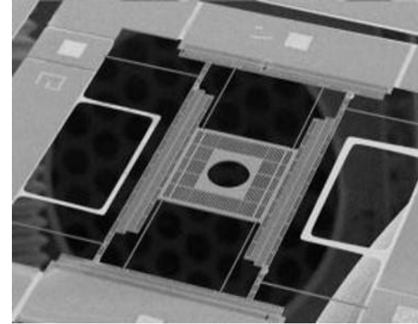
MOEMS
