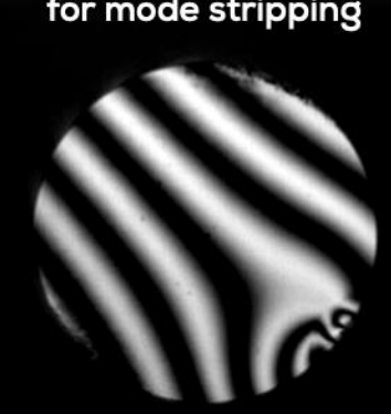
End face inspection
