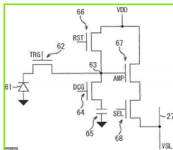
Dual Conversion Gain
