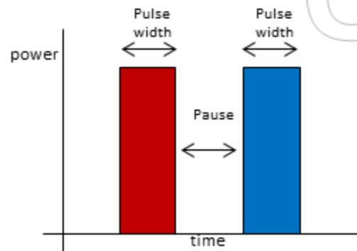
SEQUENTIAL emission of 10600 nm and 1540 nm with independent pulse width, power and variable delay between the two pulses
