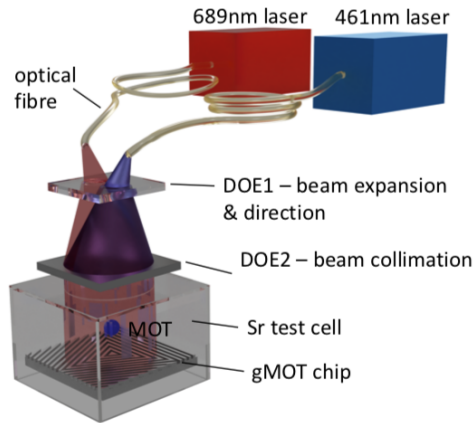
Miniature Magneto Optical Trap
